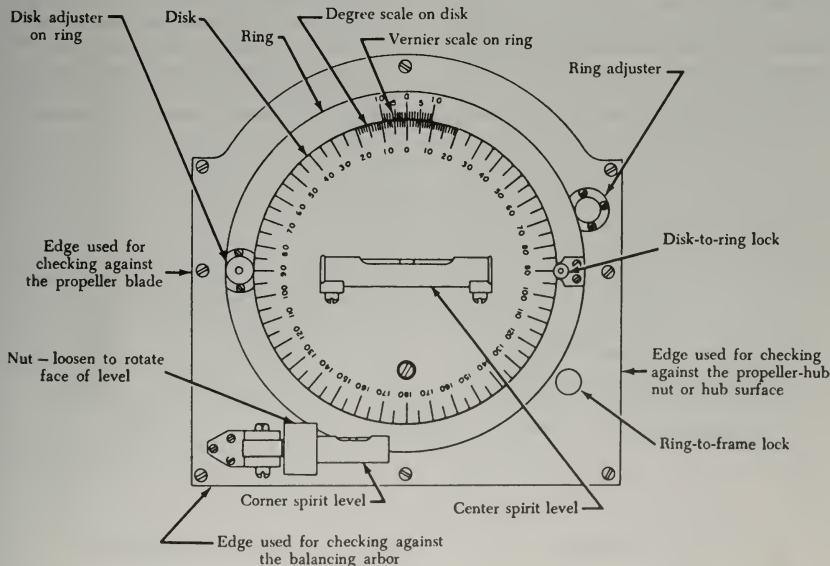
FIGURE 7-28. Universal protractor.
